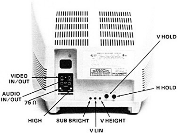
HP 82913A Video Monitor (12-inch)
